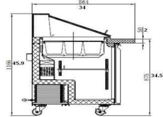
SECTION VIEW
